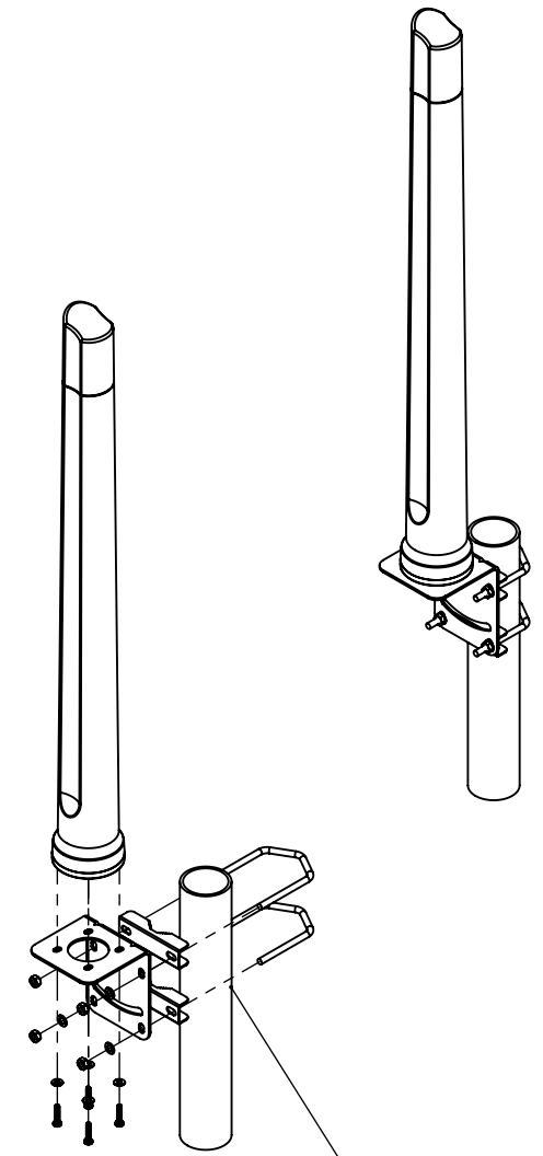
Pole Mounting Illustration
